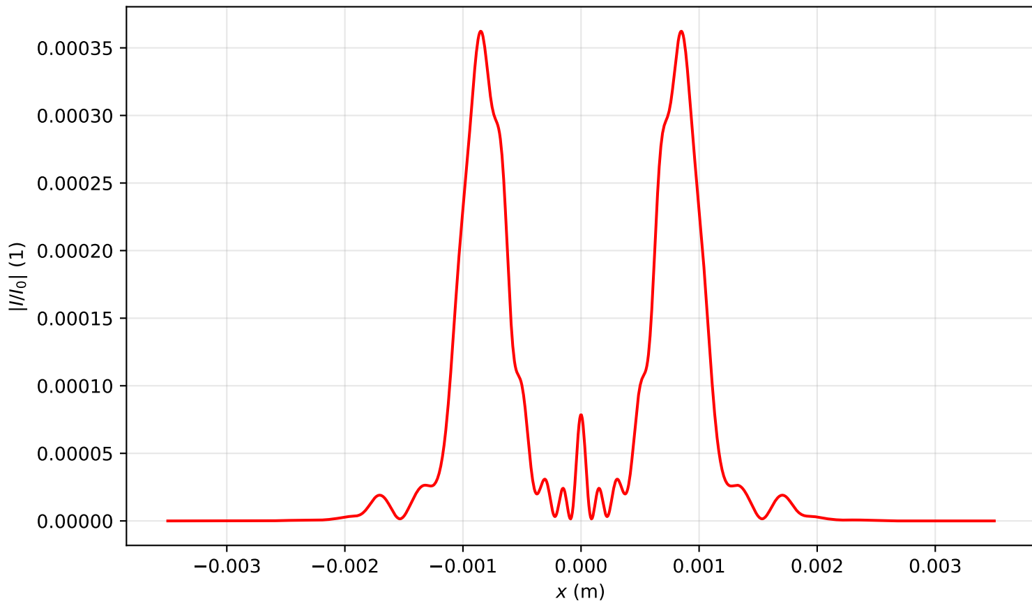
Intensity profile I(x, y = 0, z = 0.876)/I_0 , P_{in}=9.0P_{cr} , artificial time
